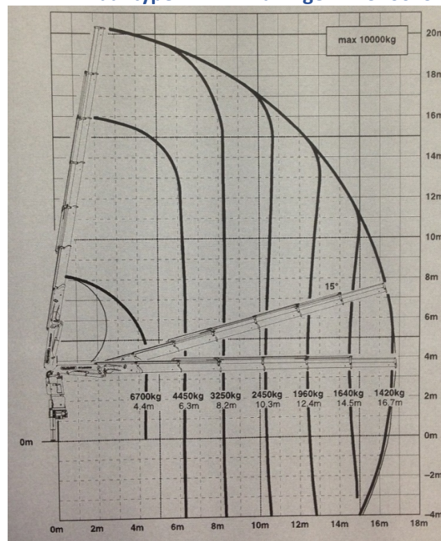
Merk: Scania Kraantype: Palfinger PK34002SH-E
